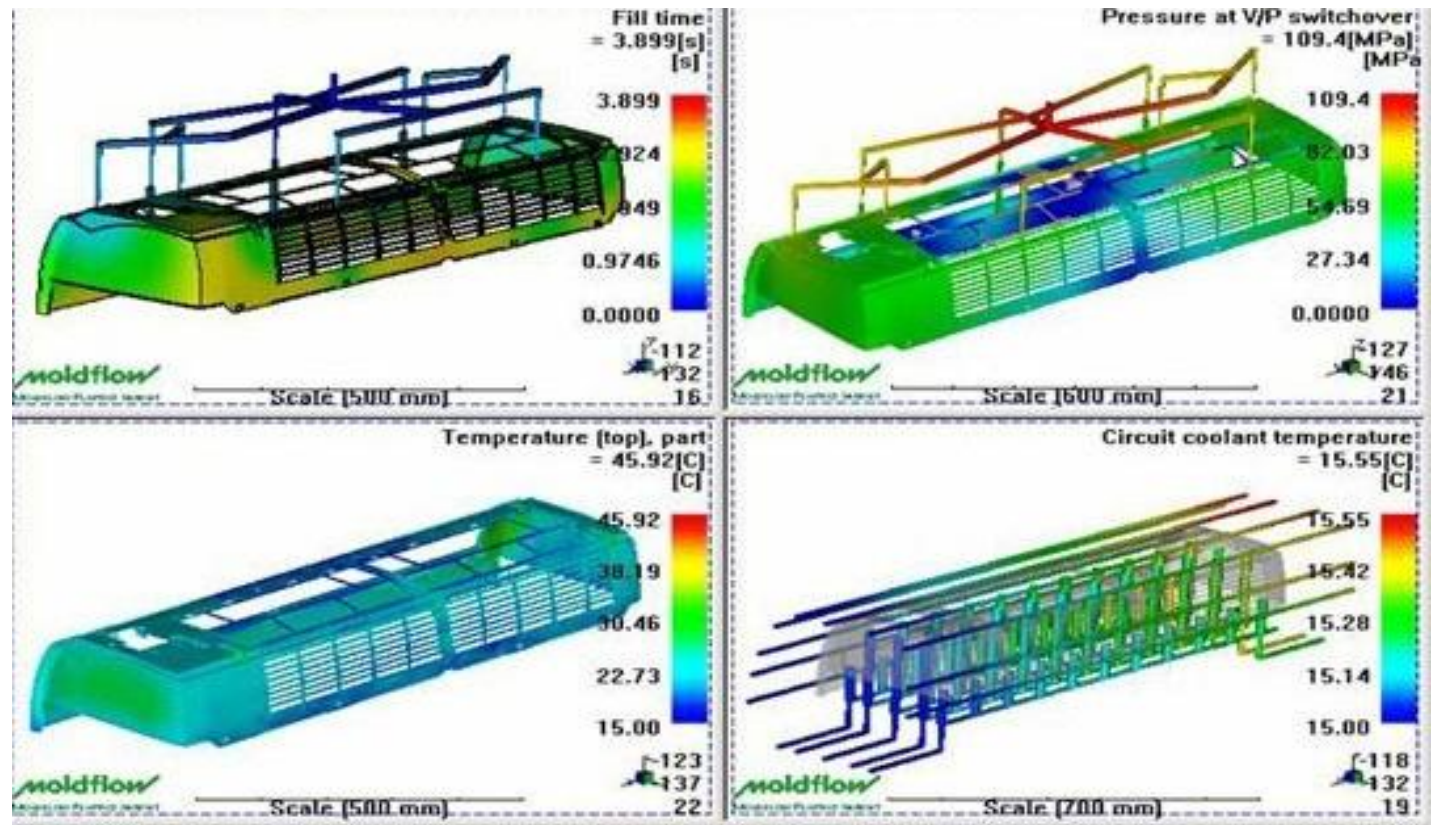
Mold Flow analysis on AC cover
